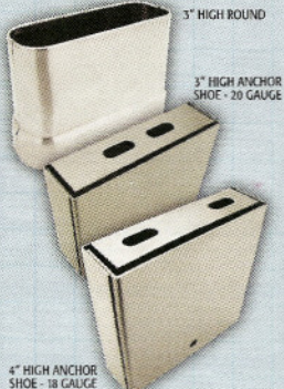
3" HIGH ROUND
